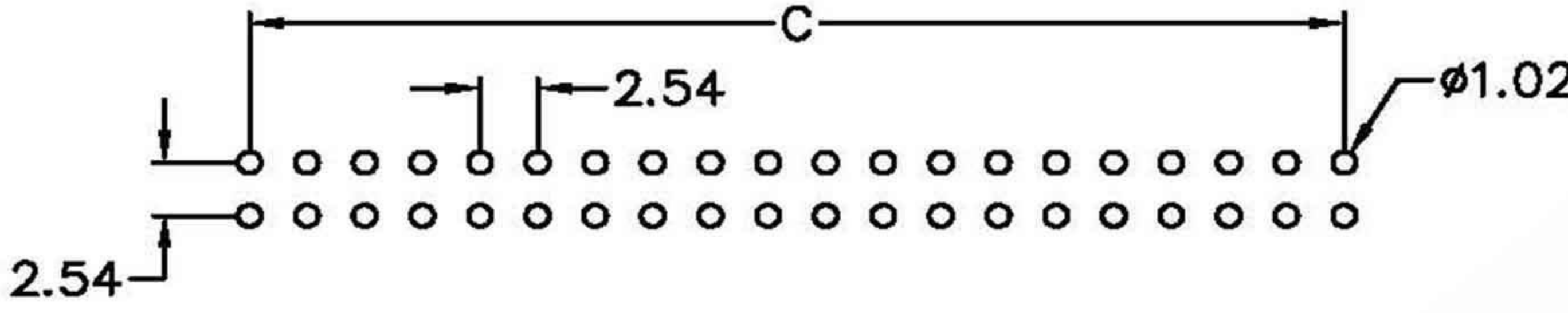
Recommended P.C.B Layout
